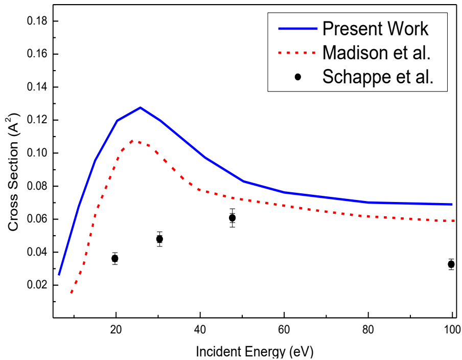
Fig. 6 Cross Section of Argon atom for transition 3p^6-3P^5s(3/2)
