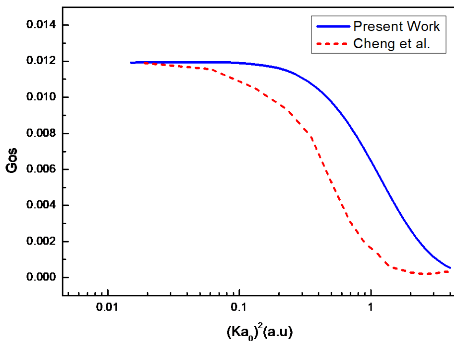
Fig. 2 Generalized oscillator strength of Neon atom for transition 2p^6-2P^5s(3/2)
