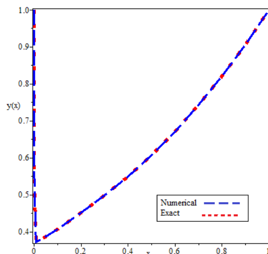
Figure 3: Comparison the exact and numerical solution ( \varepsilon = 10^{-3} and \delta = 0.1\varepsilon = \eta ) for Example 2.
