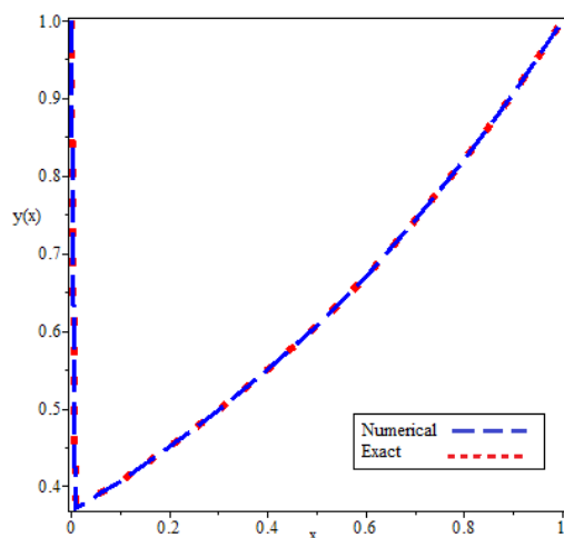
Figure 4: Comparison the exact and numerical solution ( \varepsilon = 10^{-4} and \delta = 0.1\varepsilon = \eta ) for Example 2.
