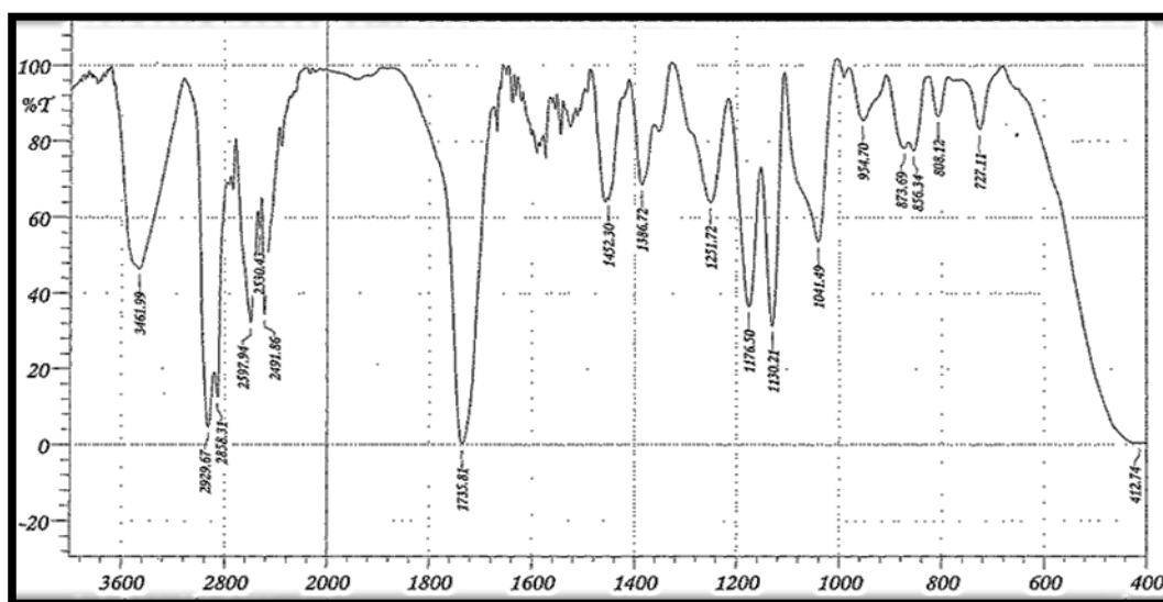
Figure (2): Infrared spectrum of poly(ethylene disbacate).
