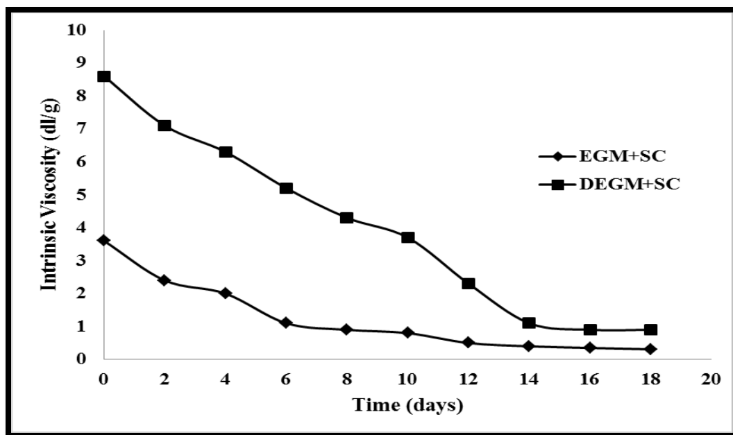
Figure (5): Influence of poly(ethylene sebacate) and poly(ethylene disbacate) biodegradation on their viscosity solutions.
