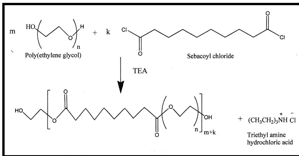
Scheme (3): Representative scheme for the synthesis of poly(ethylene glycol)-co-sebacate.
